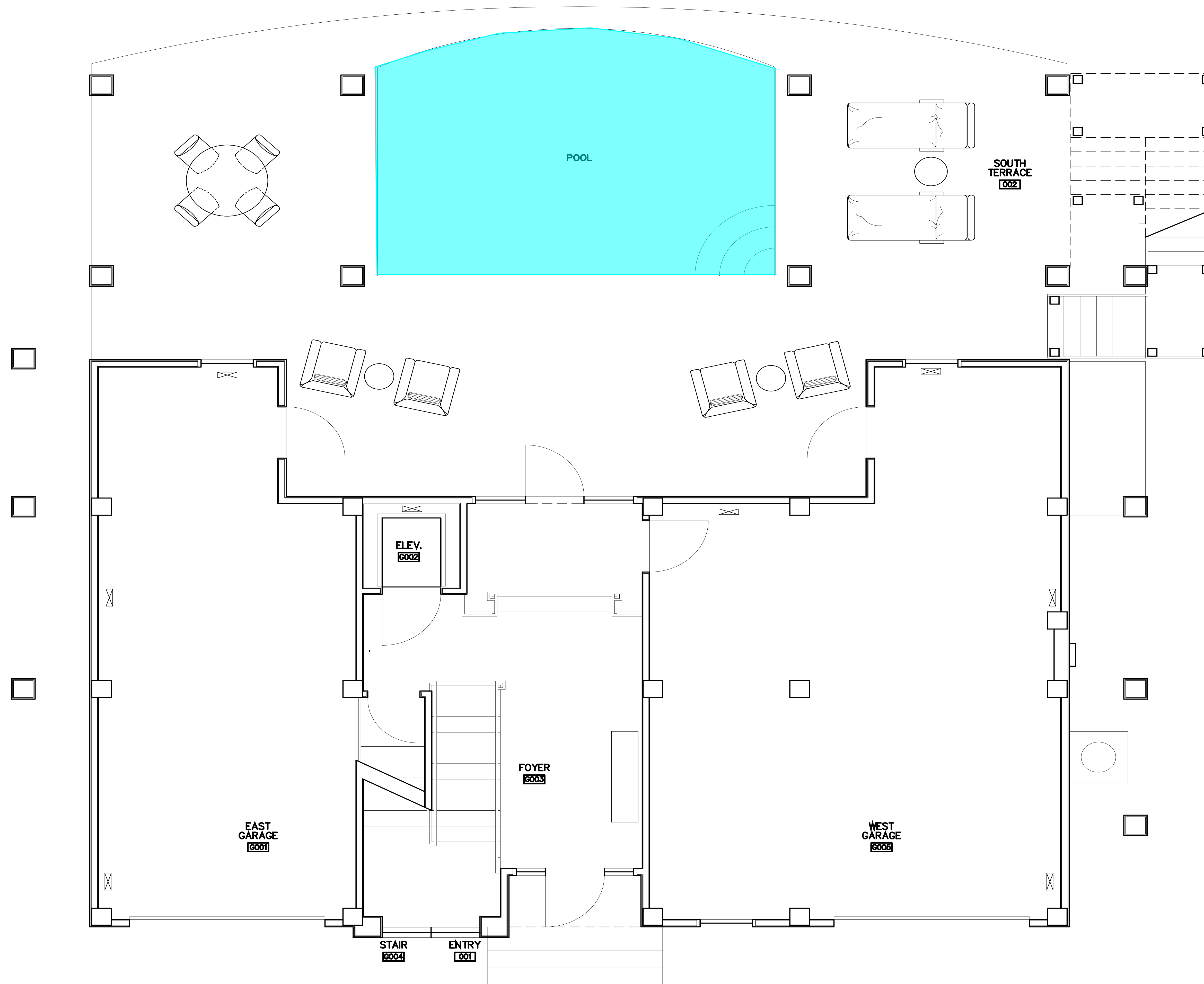
1 FURNITURE PLAN - GROUND FLOOR
